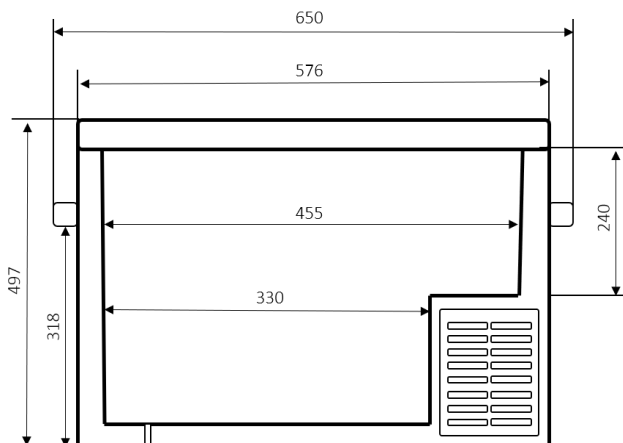
IceCube 50
